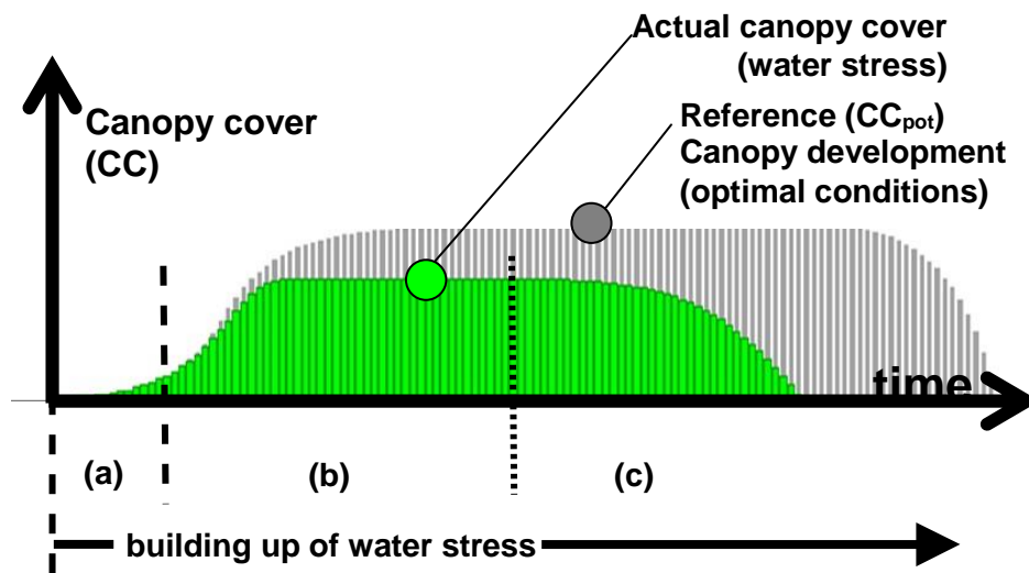
Figure 3.2.3b Simulation of the green canopy cover (CC) when water stress builds during the crop cycle with reference to the canopy development for non-stressed conditions ( CC_{pot} ). With indication of periods (a) no effect of water stress on canopy development; (b) water stress affecting leaf expansion; (c) water stress triggering early canopy decline
